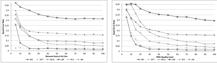
Figure 6: EER for remove lines / JPEG compression
