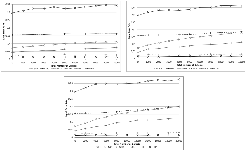
Figure 4: EER for hot, stuck and both, hot and stuck pixels combined
