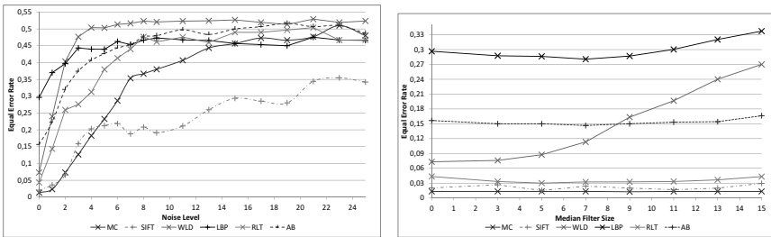
Figure 5: EER for additive noise test / median cut filtering test
