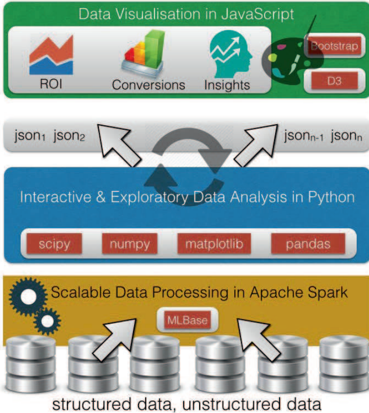
Figure 2: The RightInsight architecture for big data science depicted as a workflow.
