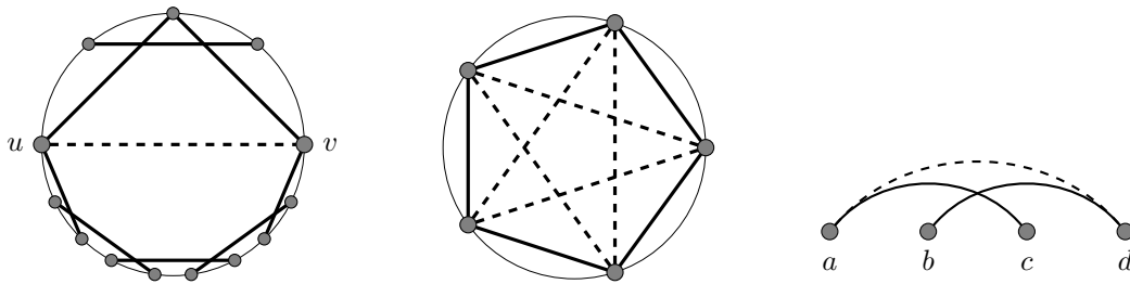
■ Figure 2 A graph in \mathcal{H} (left), an ordered hole (middle), and the forbidden configuration for a capped graph (right). Dashed lines indicate non-edges. The pairs of vertices where no lines are drawn can be edges or non-edges.
