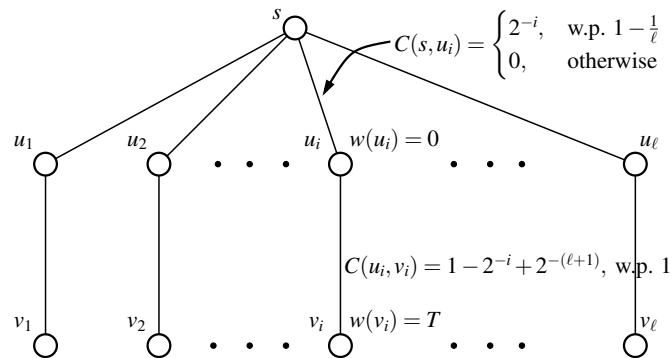
Figure 1 An instance in which the optimal adaptive strategy obtains a payoff which is \Omega(n) larger than the payoff of the optimal nonadaptive strategy.
