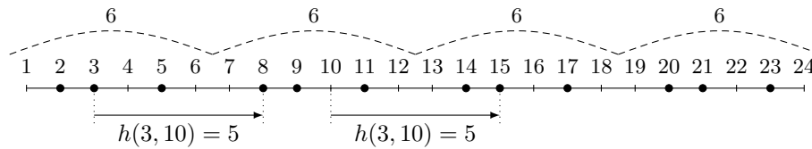
■ Figure 1 An example of a 6-cover \mathbf{S}(6) = \{2, 3, 5, 8, 9, 11, 14, 15, 19, 20, 21, 23\} (for \mathbf{D} = \{2, 3, 5\} ), with the elements marked as black circles. For example, we have h(3, 10) = 5 , since 3+5, 10+5 \in \mathbf{S}(6) .
