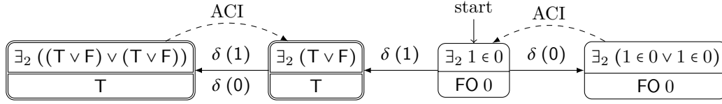
■ Figure 2 Bisimulation constructed by \text{eqv} for \exists_2 1 \in 0 \equiv FO 0 .
