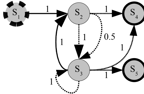
Figure 4. Social protocol presented in section 2.2 after a transition related with the action “comment a question” has been added from s_3 to s_3 .
