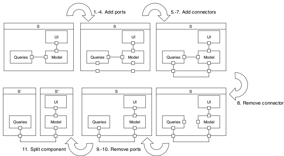
Figure 6: Complex refactoring on architectural level
