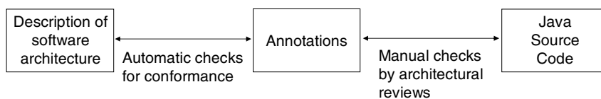
Figure 1: Architectural conformance in two steps
