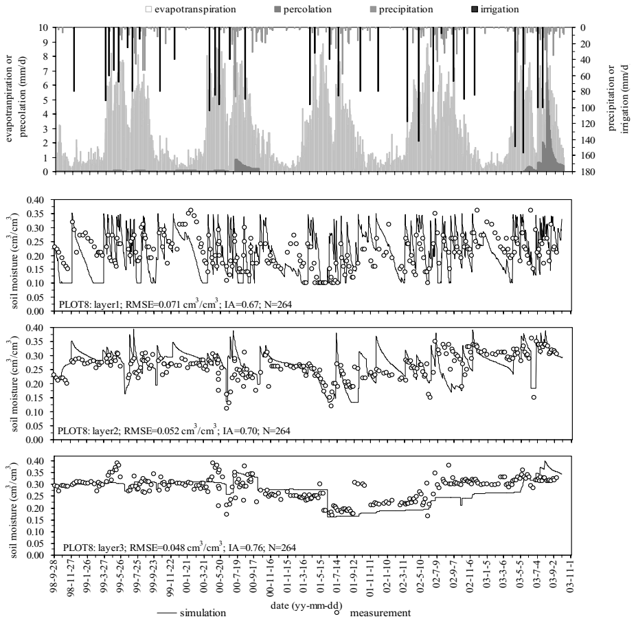
Figure 2: Seasonal dynamics of measured and simulated soil water content ( \text{cm}^3/\text{cm}^3 ), evapotranspiration, deep soil percolation, precipitation and irrigation at a irrigated plot.. RMSE= root mean square error. IA = modeling efficiency index. N = sampling number.
