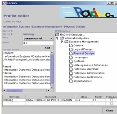
Figure 3. RACING User Profile Editor the interface for ST3 of IQ→RQ algorithm.
