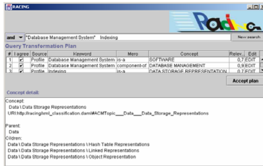
Figure 4. The interface for QP refinement and approval. Presented is the QP for the example on Fig. 1(d).
