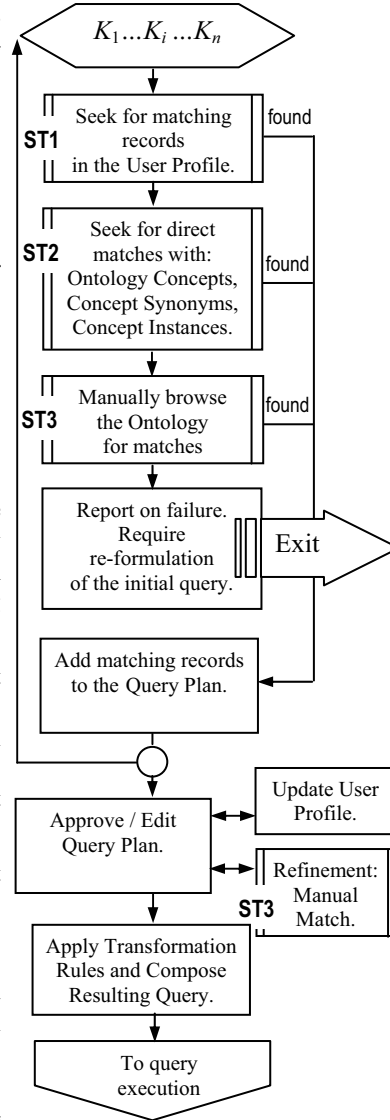
Figure 2. IQ→RQ Transformation algorithm
