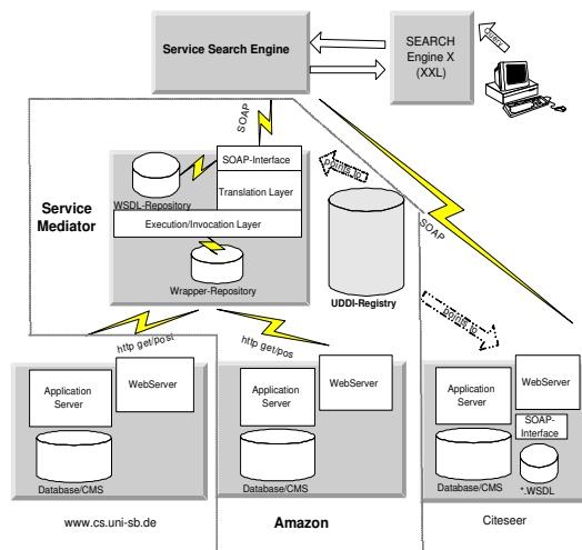
Figure 2: Service Mediator at runtime
