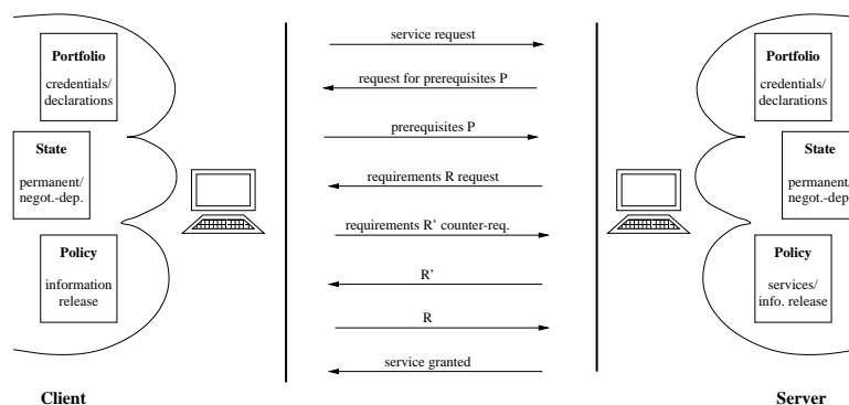
Figure 1: Client/server interplay in [BS02]
